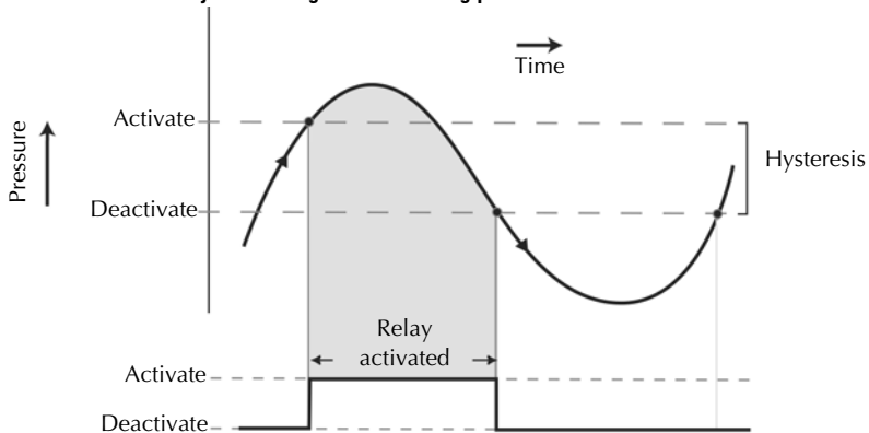
Figure 5-5 Default behavior of relays activating with increasing pressure
