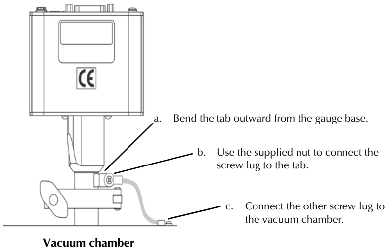
Figure 2-7 Vacuum chamber ground connections
