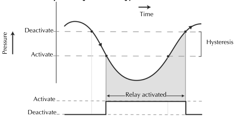
Figure 5-4 Default behavior of relays activating with decreasing pressure
