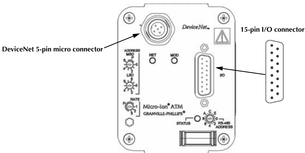
Figure 2-2 15-pin I/O connector and DeviceNet 5-pin micro connector
