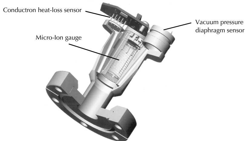
Figure C-1 Micro-Ion gauge, Conductron sensor, and pressure diaphragm sensors
