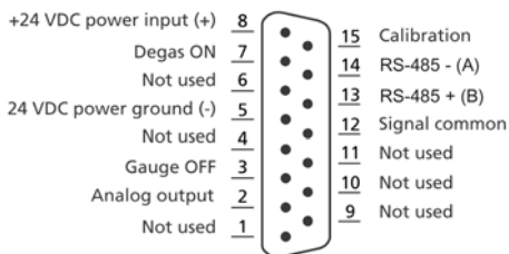
Figure 2-4 Wiring terminals for Micro-Ion ATM module with RS-485 interface, one analog output, and two trip-point relays
