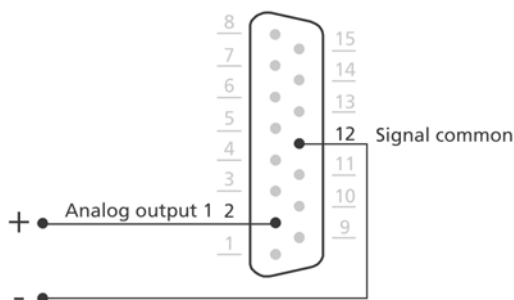
Figure 4-2 Pins 2 and 12: Voltage indicating vacuum pressure
