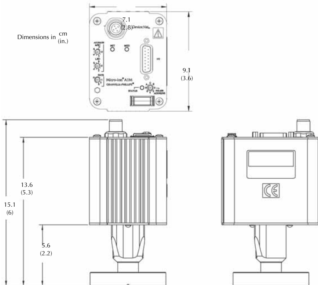
Figure 2-1 Dimensions
