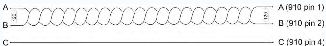
RS485 twisted pair cable run with 120 Ω terminator resistors (910 with 15 pin connector)
