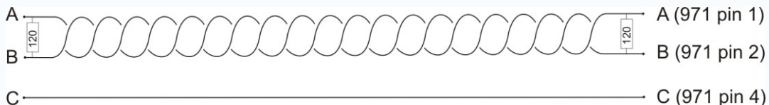
RS485 twisted pair cable run with 120 Ω terminator resistors (971 with 15 pin connector)
